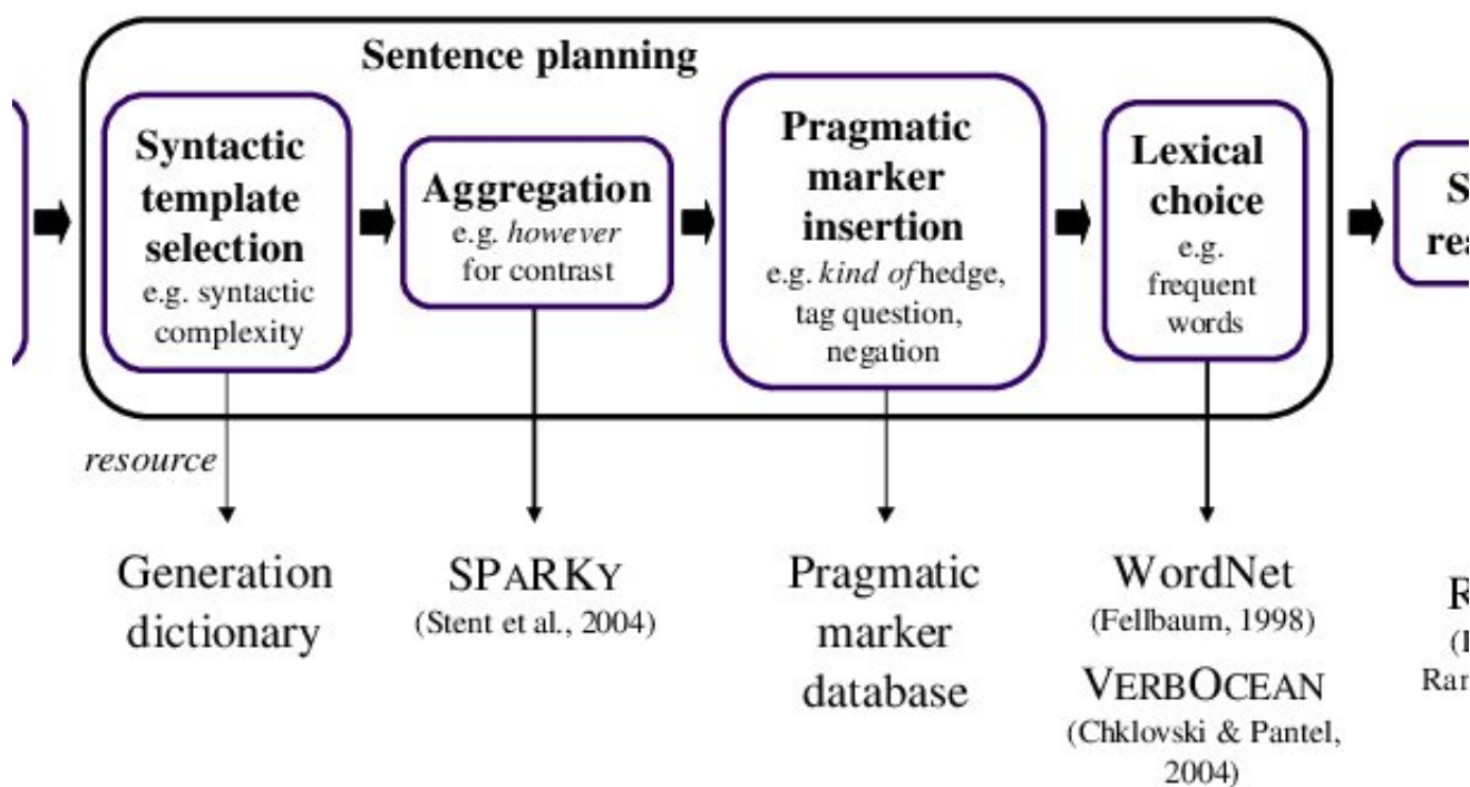
Fig. 2: The architecture of the PERSONAGE base generator.
